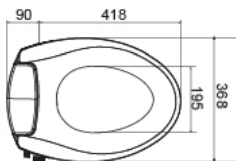
MSB-SE01 (Elongated)
