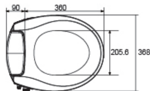
MSB-SR01 (Rounded)
